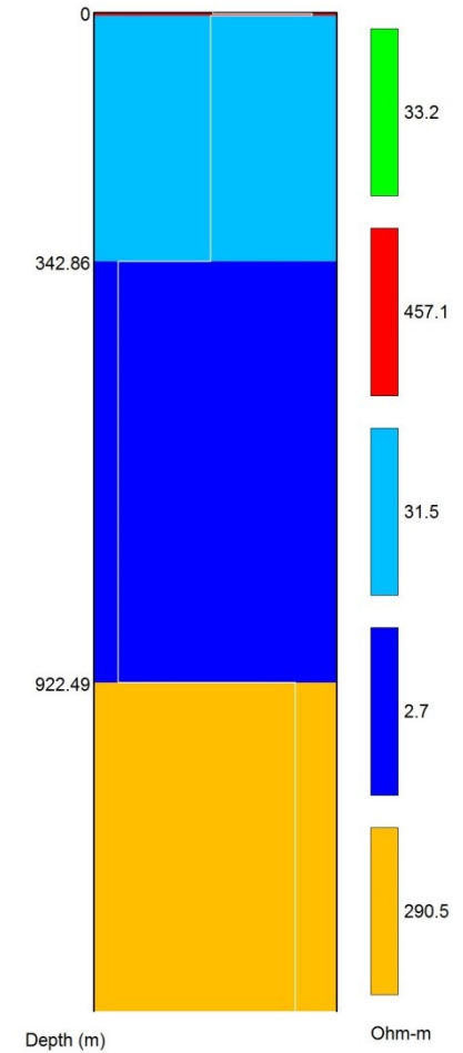
Layered Resistivity Model
