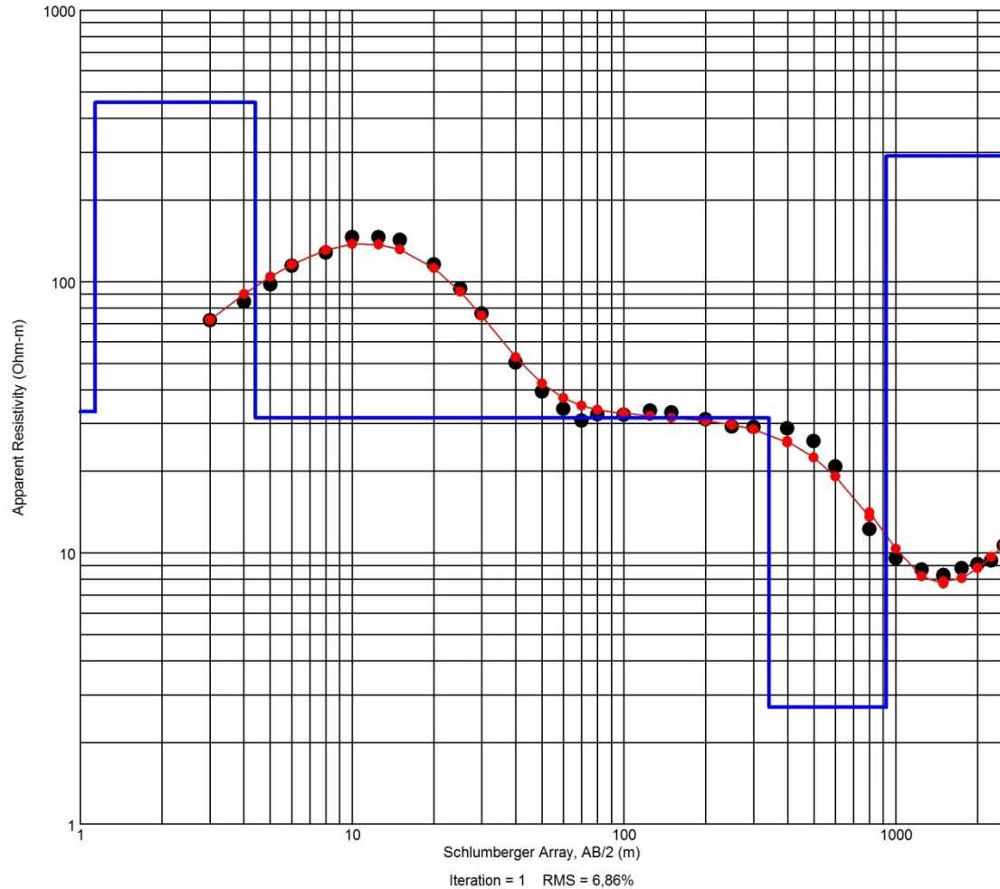
Measured and Modeled Data SEV#1
